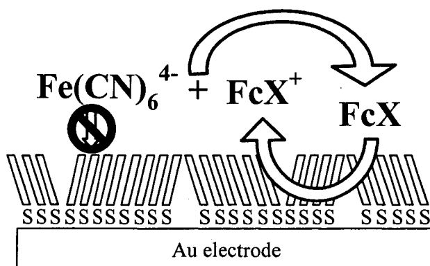
Scheme 2. Schematic representation of the amplification mechanism: electrolysis from \text{Fe}(\text{CN})_6^{4-} is suppressed, while \text{FcX} undergoes rapid oxidation. The oxidized form of the mediator ( \text{FcX}^+ ) is reduced by \text{Fe}(\text{CN})_6^{4-} back to \text{FcX} (figure adapted from Reference [4]).
