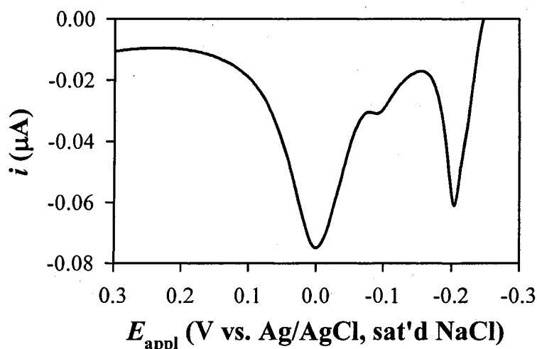
Figure 7. Stripping of underpotentially deposited lead in 1 M HClO 4 from a mechanically polished gold disk electrode. Geometric electrode area: 0.020 cm 2 , R_f : 1.3, and sweep rate: 20 mV s -1 .
